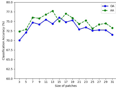
Fig. 9. Classification results of different patch sizes on the Indian Pine dataset.
