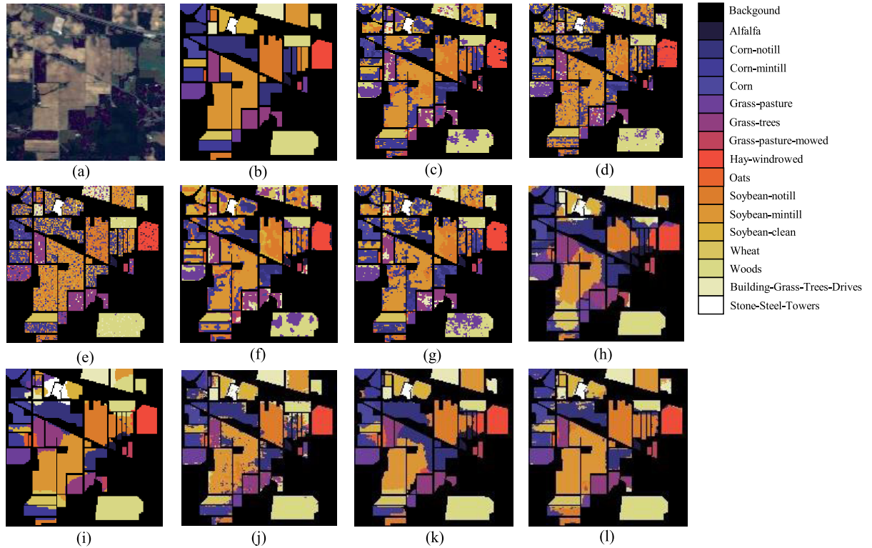
Fig. 5. Classification maps of different methods on the Indian Pines dataset. (a) Pseudo-color image. (b) Ground-truth map. (c) EMP + SVM (OA: 56.80%). (d) TSVM (OA: 57.65%). (e) JCR (OA: 64.95%). (f) 3-D-CAE (OA: 52.21%). (g) GAN (OA: 60.24%). (h) ResNet50 (OA: 66.05%). (i) DMVL (OA: 78.01%). (j) EADNet (OA: 65.97%). (k) SC-ResNet50 (OA: 78.76%). (l) SC-EADNet (82.69%).
