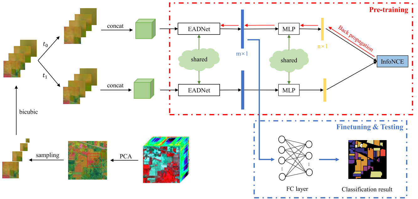
Fig. 1. Overview of the proposed SC-EADNet. t_0 and t_1 represent two branches of data augmentation used to generate different views for self-supervised contrastive learning. We use EADNet to extract representation vectors of length m \times 1 for each patch and use MLP to project the representation vectors to length n \times 1 . InfoNCE is the optimization objective of the pretraining stage. The parameters of EADNet and MLP are shared between two branches. Classification is performed through an FC layer.
