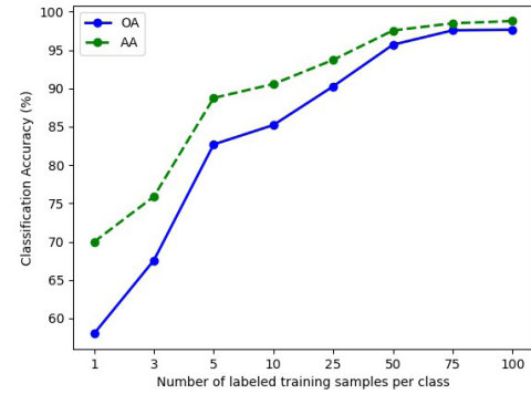
Fig. 11. Classification results of different number of labeled training samples on the Indian Pine dataset.
