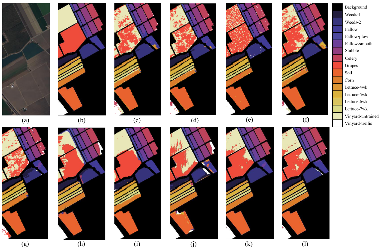
Fig. 6. Classification maps of different methods on the Salinas dataset. (a) Pseudo-color image. (b) Ground-truth map. (c) EMP + SVM (OA: 83.47%). (d) TSVM (OA: 85.63%). (e) JCR (OA: 84.93%). (f) 3-D-CAE (OA: 52.21%). (g) GAN (OA: 81.67%). (h) ResNet50 (OA: 85.98%). (i) DMVL (OA: 94.60%). (j) EADNet (OA: 80.23%). (k) SC-ResNet50 (OA: 94.18%). (l) SC-EADNet (94.73%).
