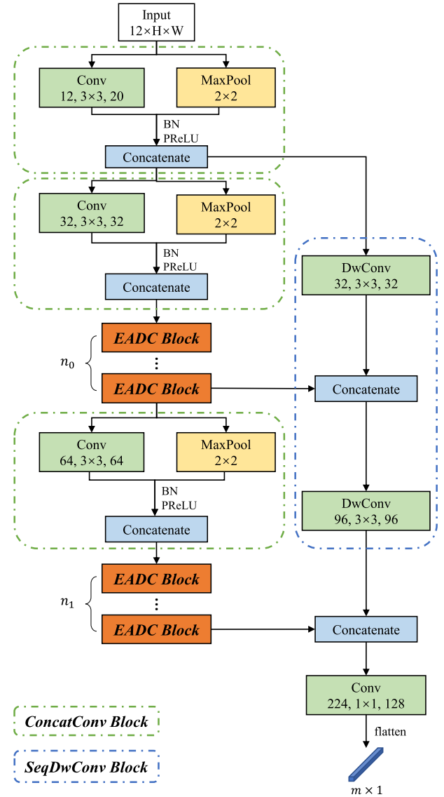
Fig. 3. Overview of the proposed EADNet. In the figure, DwConv means depthwise convolution, and n_i represents the repetitive number of EADC blocks. ConcatConv block is used for the backbone FE and downsampling. SeqDwConv block unifies the feature maps in shallow layers and concatenates them with the deep layers for FE. Best viewed in color.
