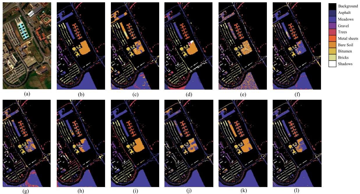
Fig. 7. Classification maps of different methods on the PaviaU dataset. (a) Pseudo-color image. (b) Ground-truth map. (c) EMP + SVM (OA: 70.77%). (d) TSVM (OA: 71.62%). (e) JCR (OA: 70.90%). (f) 3-D-CAE (OA: 70.85%). (g) GAN (OA: 72.06%). (h) ResNet50 (OA: 83.47%). (i) DMVL (OA: 86.96%). (j) EADNet (OA: 82.21%). (k) SC-ResNet50 (OA: 89.98%). (l) SC-EADNet (OA: 85.06%).
