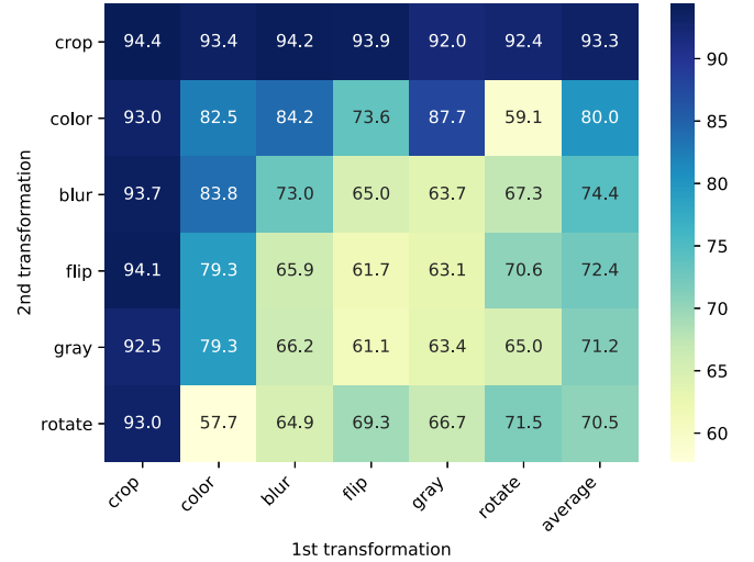
Fig. 2. Linear evaluation results on the Indian Pines dataset under individual or pairwise combination of data augmentation. The last column denotes the average value over each row. Best viewed in color.
