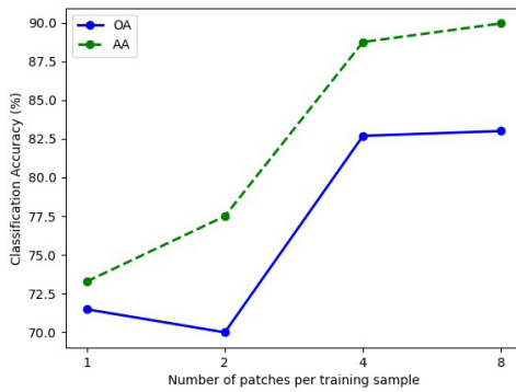
Fig. 10. Classification results of different number of input patches on the Indian Pine dataset.
